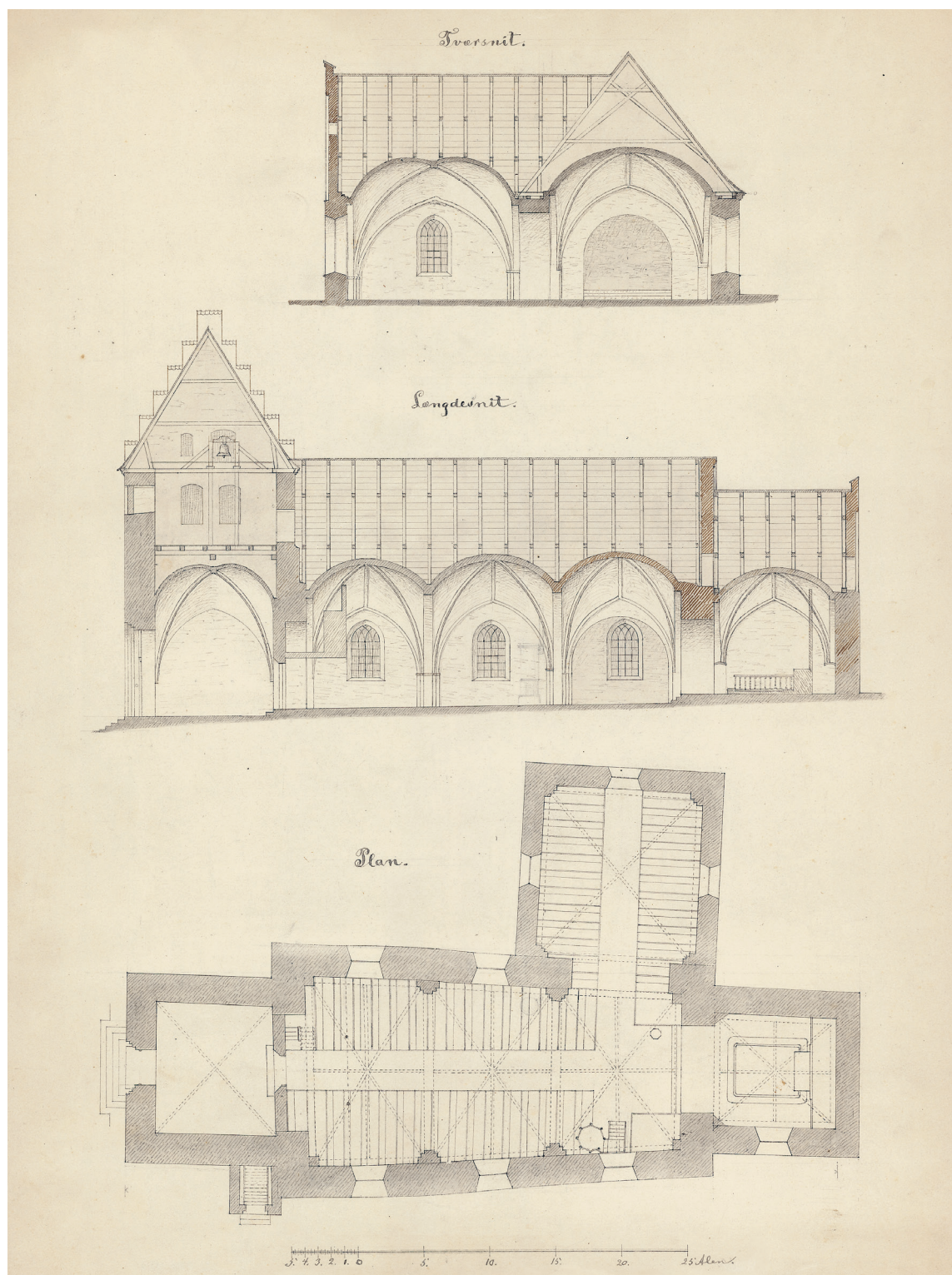
Fig. 12a-c. Opmåling af kirken o. 1880. 1:300. a. Tversnit set mod øst. b. Længdesnit set mod nord. c. Grundplan. I NM. — Scale drawings of the church from c. 1880. a. Cross-section looking east. b. Longitudinal section looking north. c. Ground plan.
